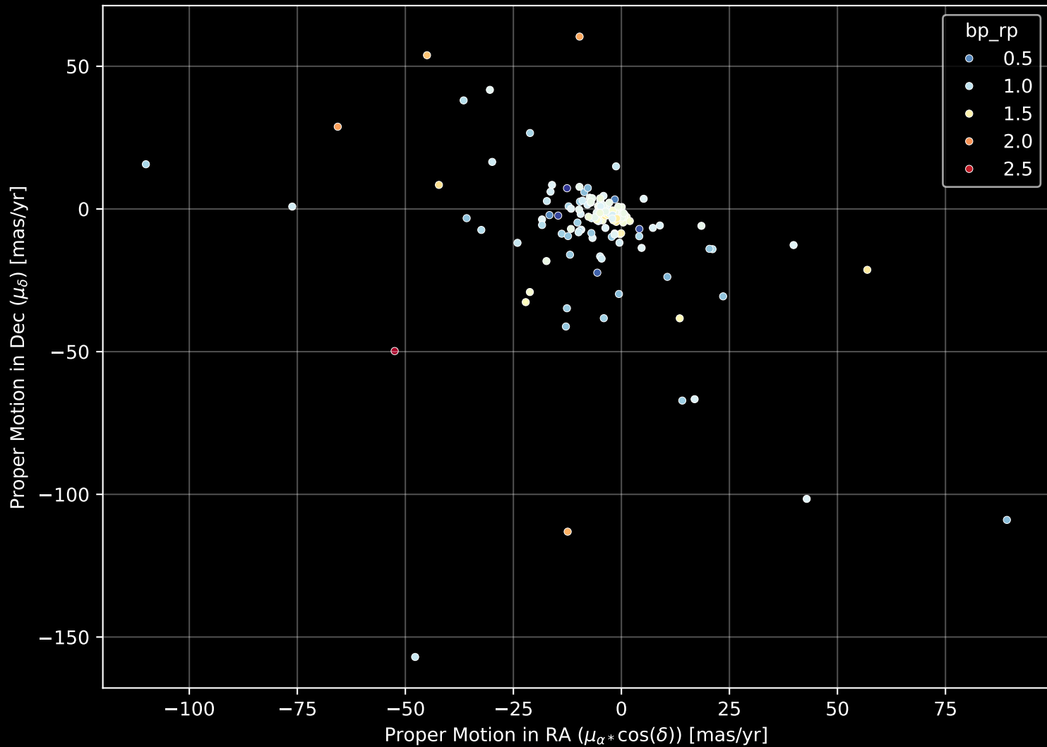
APOGEE DR17 Field: [225+29_MGA] Proper Motion Diagram (n= 145)
