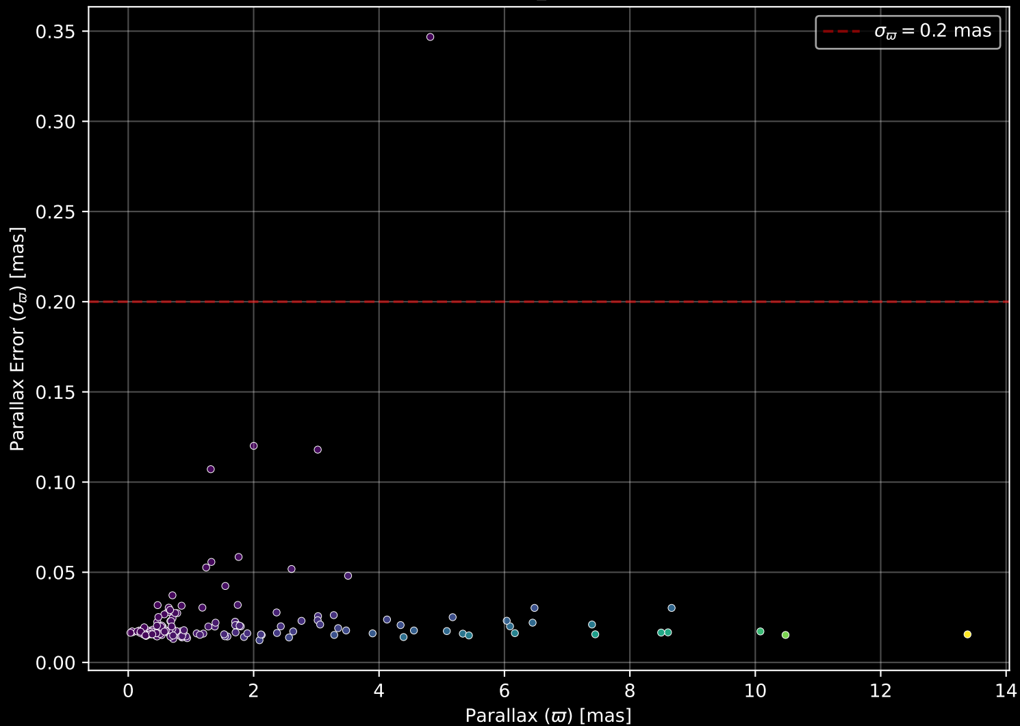
APOGEE DR17 Field: [225+29_MGA] Parallax Quality (n= 145)
