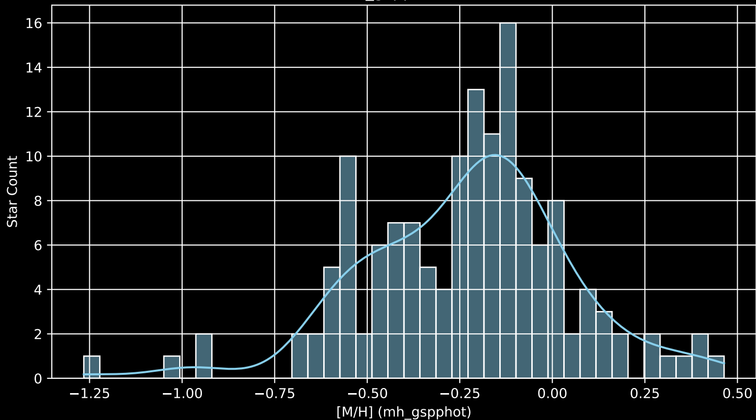
APOGEE DR17 Field: [225+29_MGA [M/H] (mh_gspphot) (n= 145)
