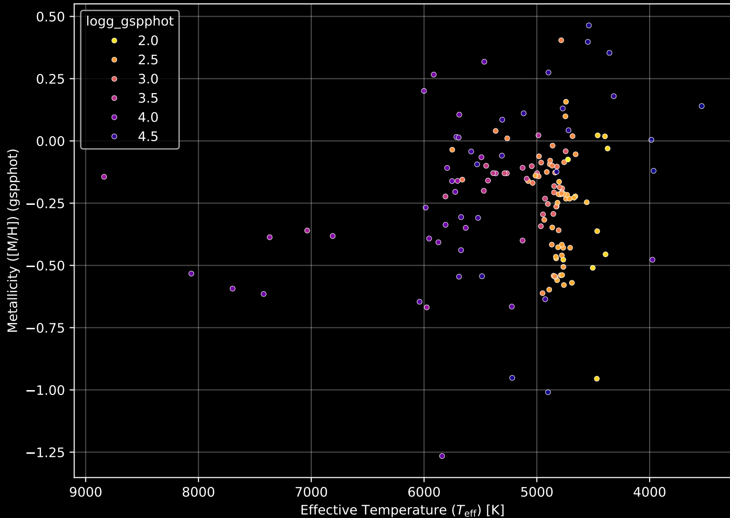
APOGEE DR17 Field: [225+29_MGA] Stellar Population Parameters (n= 145)
