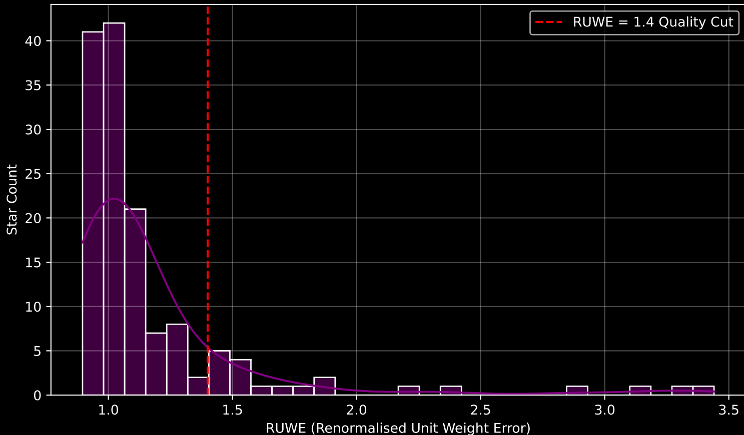
GAPOGEE DR17 Field [225+29_MGA] RUWE Distribution (n= 141)
