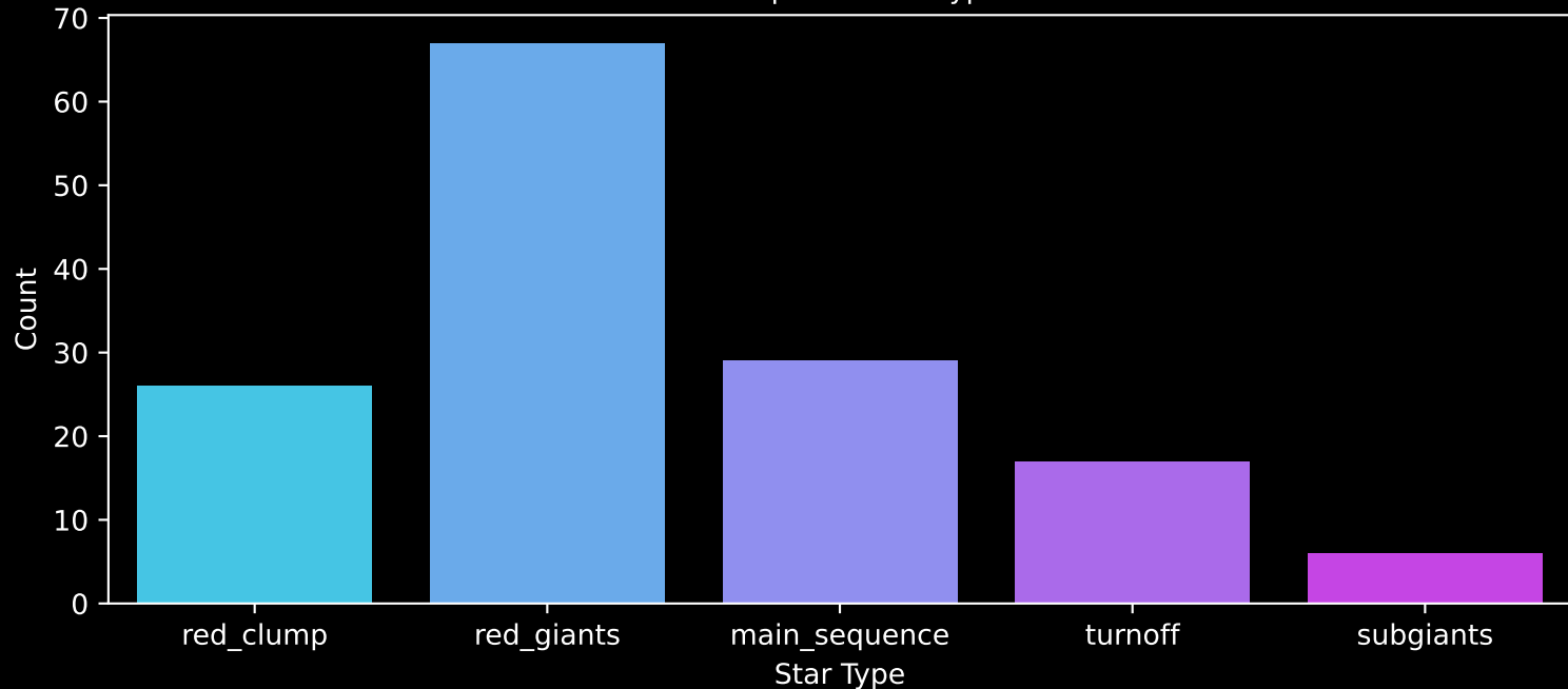
APOGEE DR17 Field: [225+29_MGA] Count plot of Star Type
