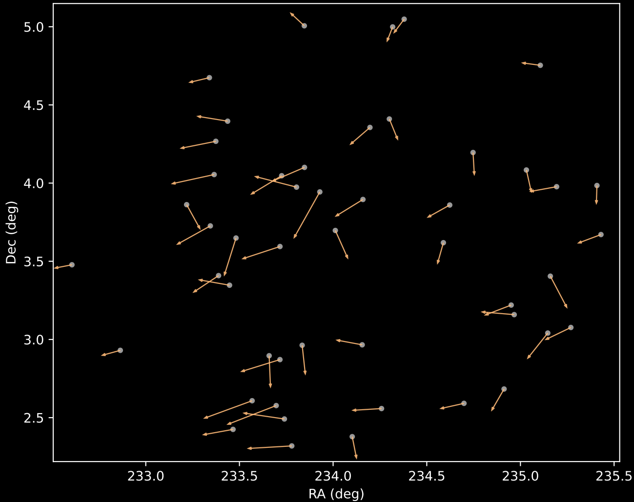
APOGEE DR17 Cluster 3 Proper Motion Vectors (n=49)
